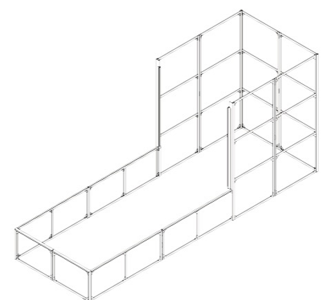
Frame - Back Right Isometric
